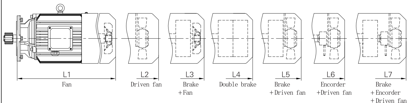
Corresponding motor dimension table for C216/C316
