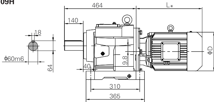
Horizontal foot-mounted
