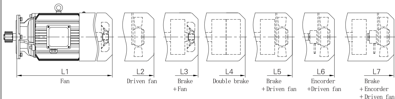
Corresponding motor dimension table for C212/C312
