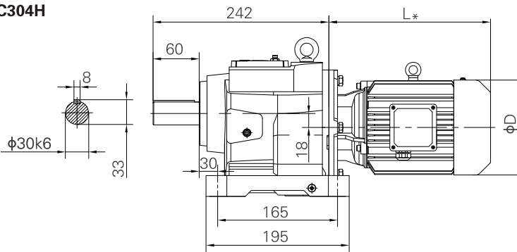
Horizontal foot-mounted
