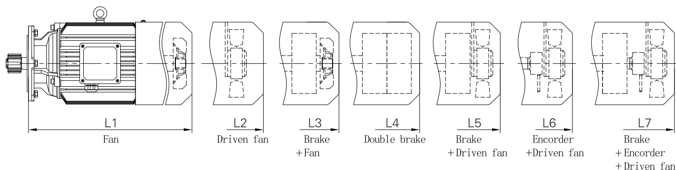
Corresponding motor dimension table for C203/C303
