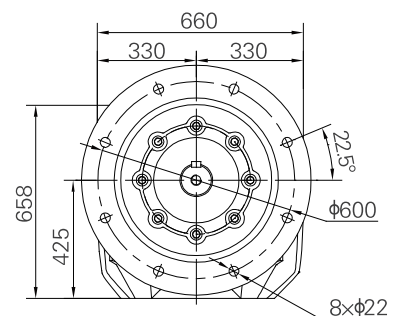
Weight: 645kg ( Without motor and oil )
