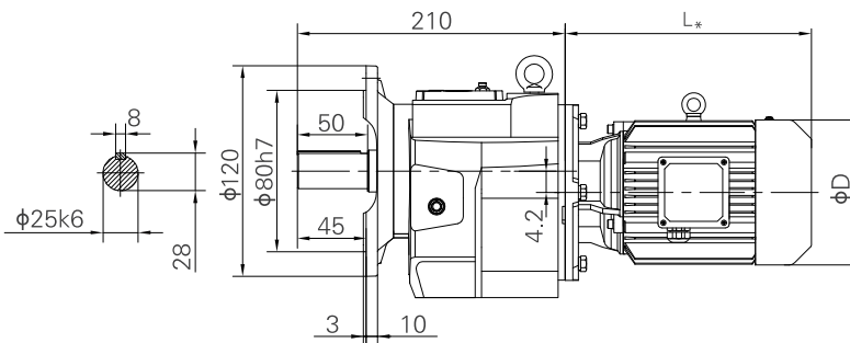
Short flange-mounted
