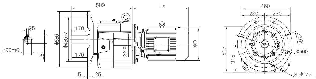
Flange-mounted
