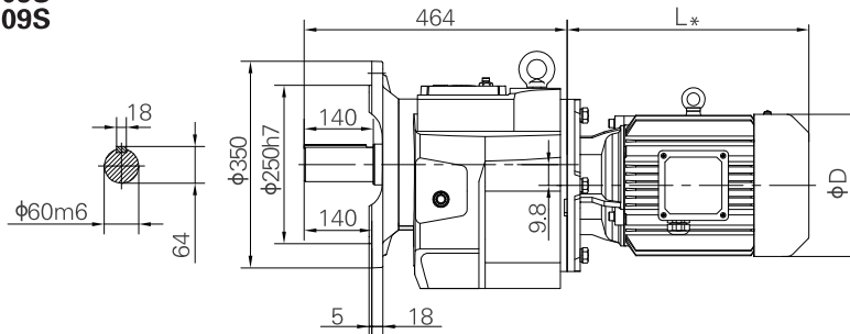
Short flange-mounted
