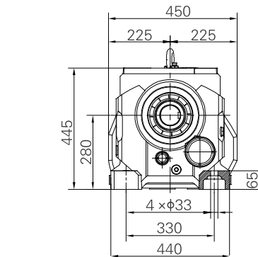
Weight: 175kg ( Without motor and oil )
