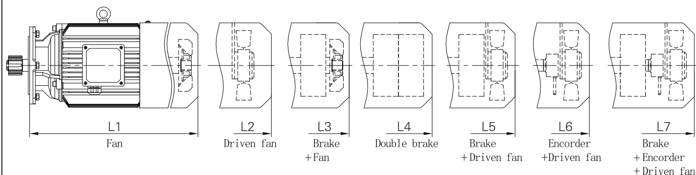
Corresponding motor dimension table for C209/C309
