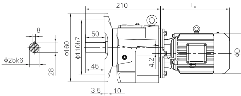
Flange-mounted
