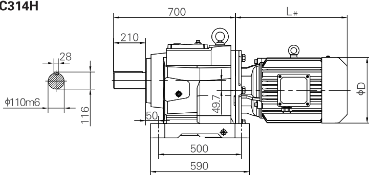
Horizontal foot-mounted
