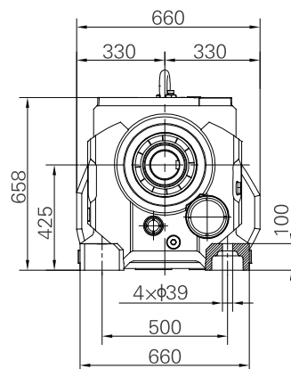
Weight: 615kg ( Without motor and oil )
