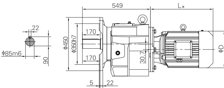
Short flange-mounted
