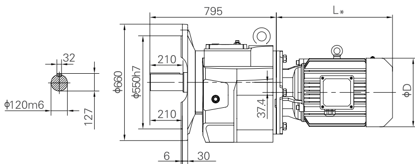
Flange-mounted
