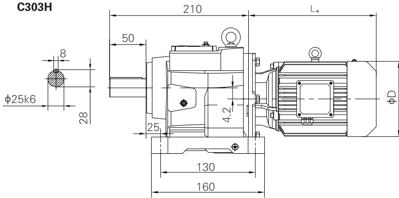
Horizontal foot-mounted
