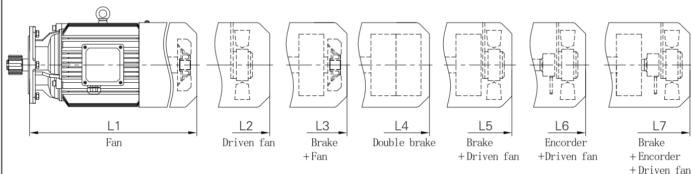
Corresponding motor dimension table for C206/C306
