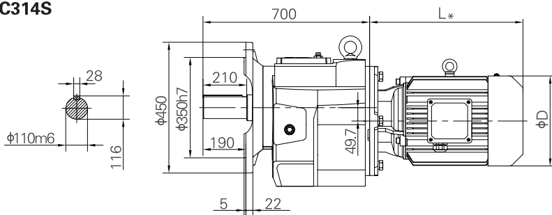
Short flange-mounted
