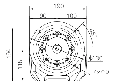
Weight: 19kg ( Without motor and oil )
