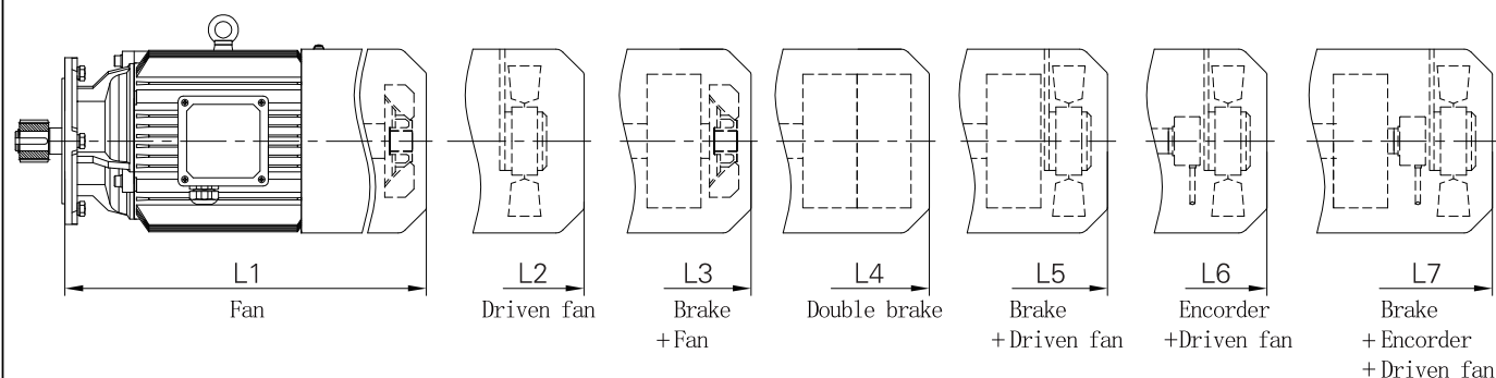
Corresponding motor dimension table for C204/C304
