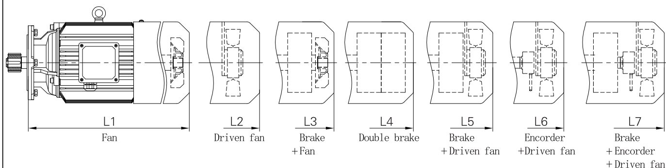
Corresponding motor dimension table for C214/C314
