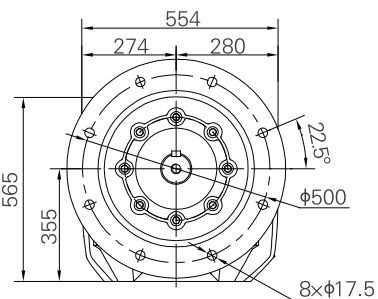
Weight: 395kg ( Without motor and oil )
