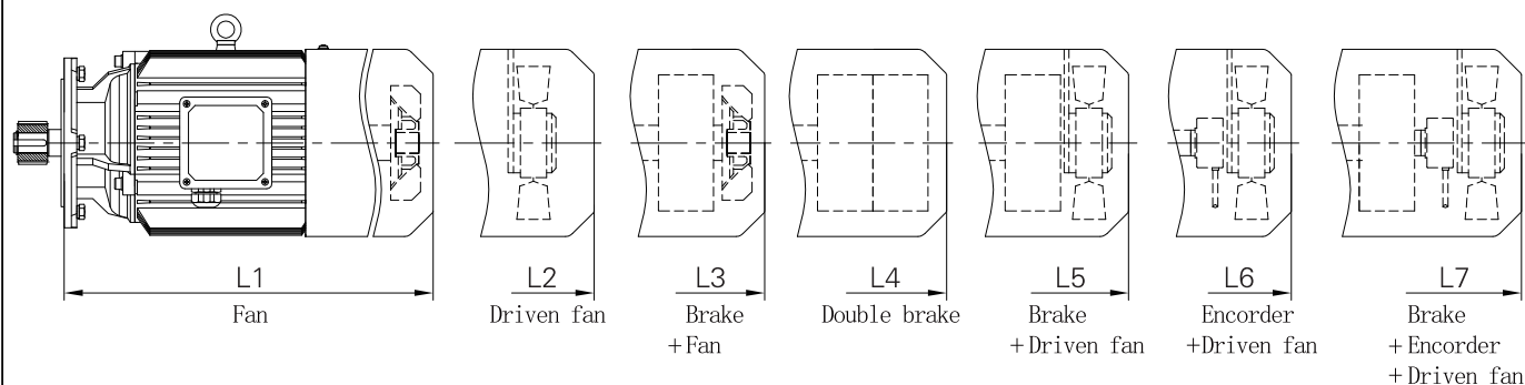
Corresponding motor dimension table for C210/C310
