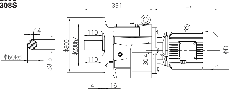
Short flange-mounted
