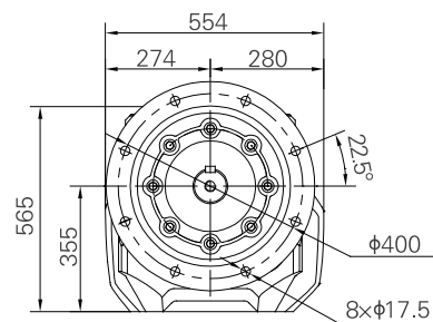
Weight: 380kg ( Without motor and oil )
