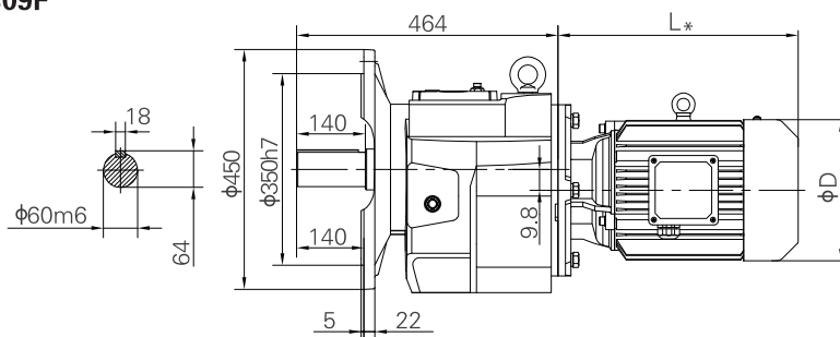
Flange-mounted
