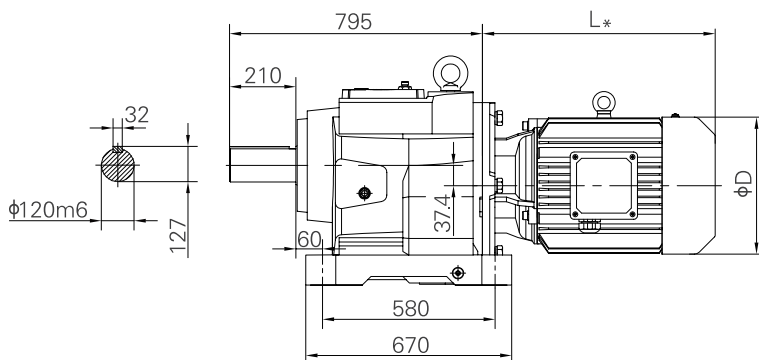
Horizontal foot-mounted
