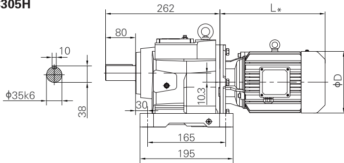
Horizontal foot-mounted
