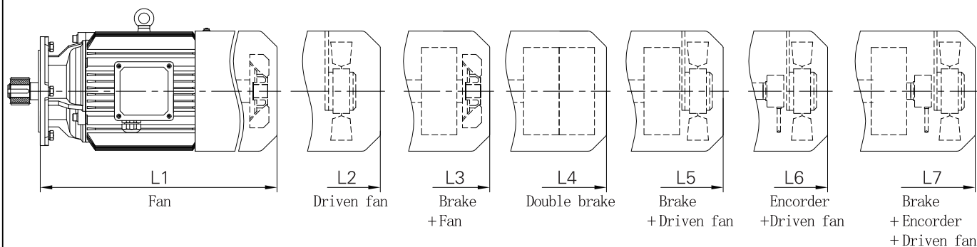
Corresponding motor dimension table for C207/C307
