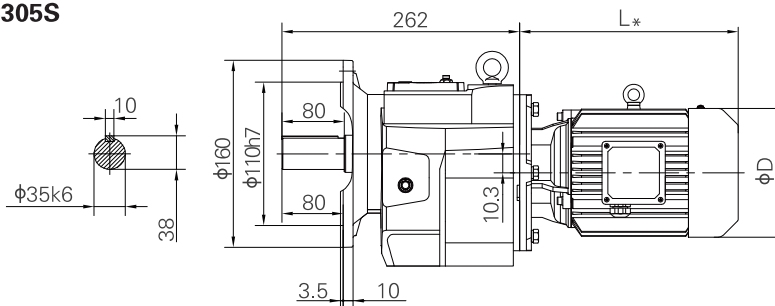
Short flange-mounted
