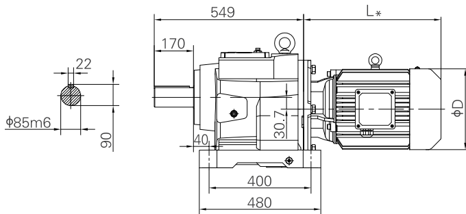
Horizontal foot-mounted
