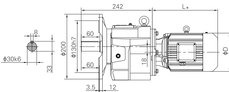
Flange-mounted
