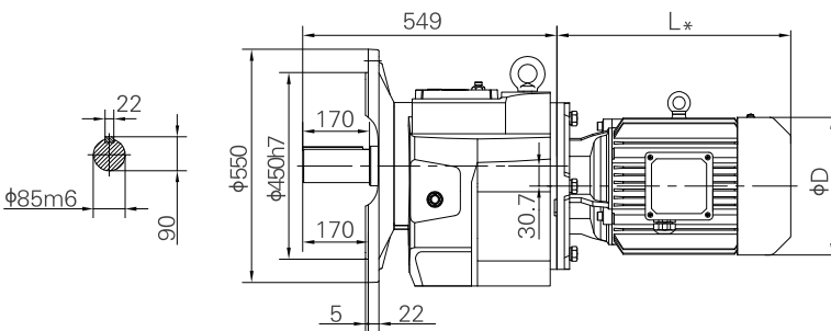
Flange-mounted
