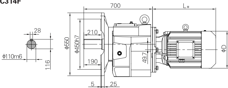
Flange-mounted
