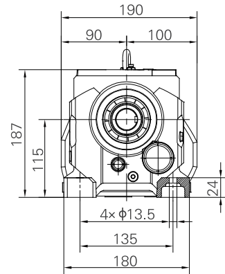
Weight: 18kg ( Without motor and oil )
