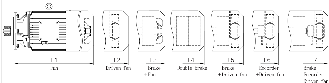
Corresponding motor dimension table for C205/C305
