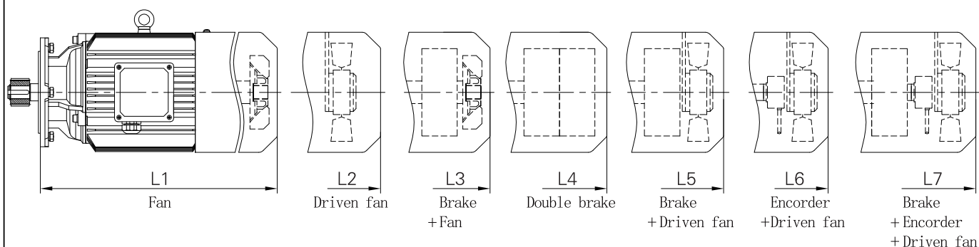
Corresponding motor dimension table for C208/C308
