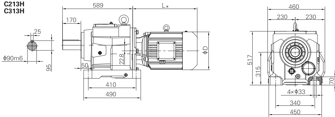
Horizontal foot-mounted
