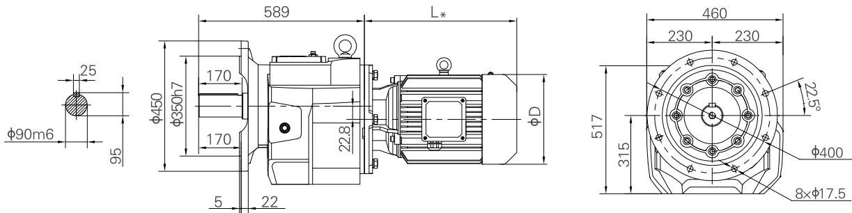
Short flange-mounted
