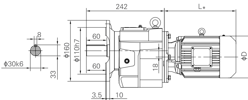
Short flange-mounted
